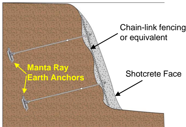
TYPICAL HILLSIDE SLOPE STABILISATION
